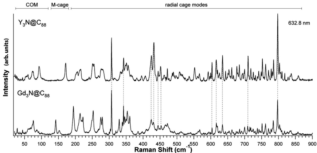
FIG. 6. Comparison of Y 3 N@C 88 and Gd 3 N@C 88 Raman data taken at 90 K. Analysis of the data identifies C 88 cage modes, hindered rotation modes and center-of-mass modes. Prominent peak correlations are denoted by dotted lines.
