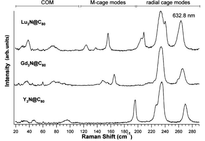
FIG. 5. Comparison of Y 3 N@C 80 , Gd 3 N@C 80 , and Lu 3 N@C 80 low-energy Raman data taken at 90 K. Analysis of the data identifies C 80 cage modes, hindered rotation modes, and center-of-mass modes.
