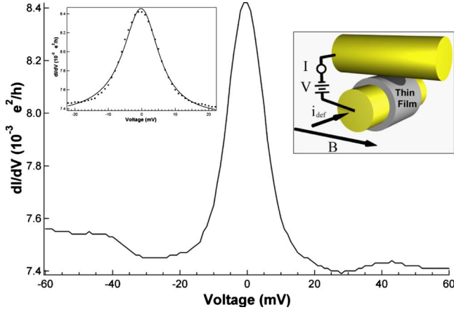
FIG. 7. (Color online) Experimental conductance data of Kondo effect and zero-bias anomaly in \text{Gd}_3\text{N}@C_{80} taken at 4.2 K. Right inset adapted from Ref. 42 shows the experimental setup: Au crossed-wire apparatus forms a junction with the \text{Gd}_3\text{N}@C_{80} thin film. Left inset shows the calculated fit (solid line) using the Fano model.
